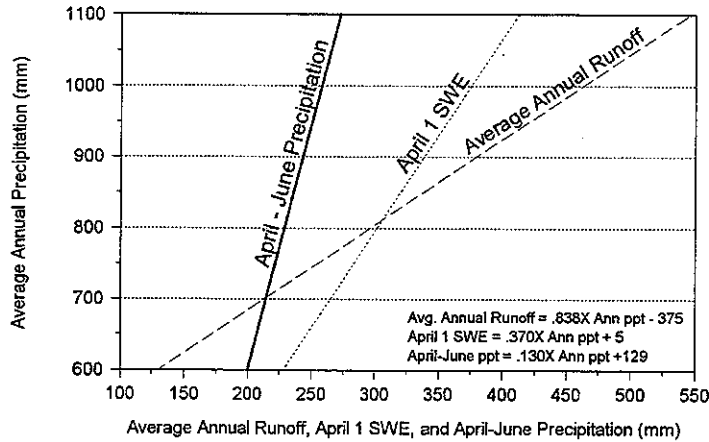
Figure 1. Average annual precipitation versus runoff, April 1 snow water equivalent (SWE) and April - June precipitation in open canopy areas on the Tenderfoot Creek Experimental Forest.
