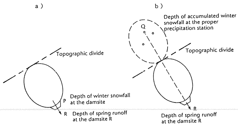
Fig.-2 Model of a combination of a valley and a river basin where the snow is split over the topographic divide. (a) River basin (b) Combination of a valley and a river basin
