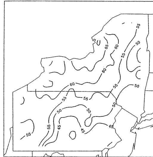
Figure 7. The percentage of total January snowfall attributed to the four "lake snow" synoptic types.
