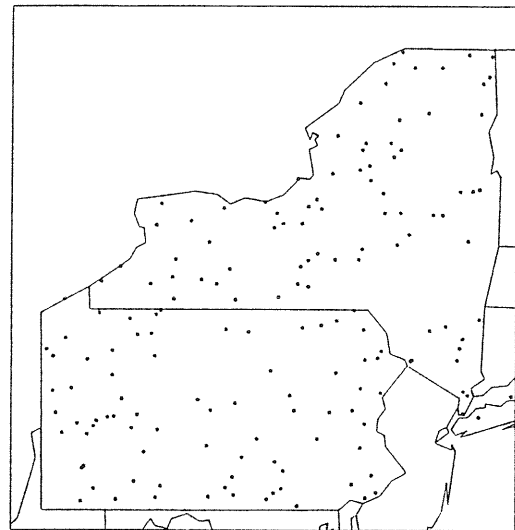
Figure 2. Distribution of stations with daily snowfall observations.
