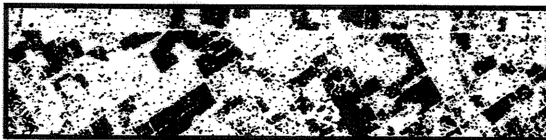
Figure 6: Classified RADARSAT C-VV image for site 2 - snowcovered areas are white
