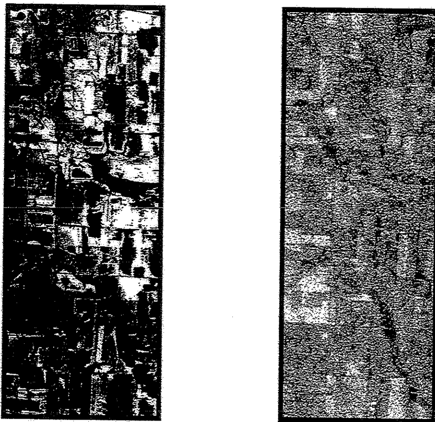
(a) Ground reference map - snowcovered areas are white
