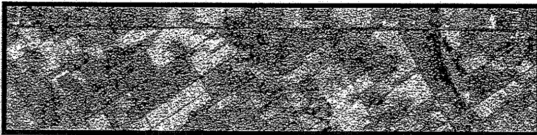
(b) Raw RADARSAT C-VV image - snowcovered areas are generally dark gray to black
