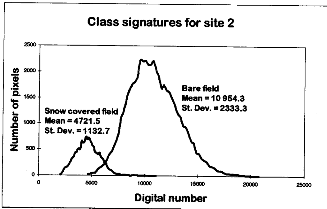
Figure 4: Class signatures for site 1 and site 2
