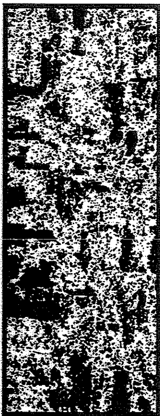
Figure 5: Classified RADARSAT image for site 1 - snowcovered areas are white
