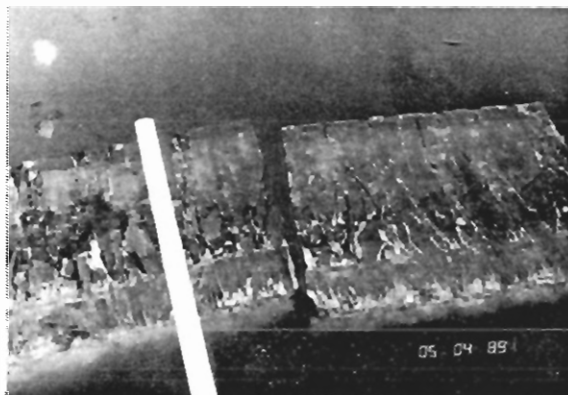
Fig. 8 Failed beam specimen after removal from test frame. Face shown represents the beam depth with the top surface towards the bottom of the photograph. Note the vertically regressive porous structure.
