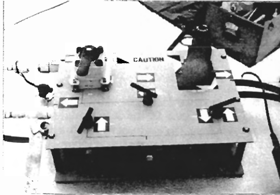
Fig. 4 Load/flow control console showing the pressure compensated flow control installed.
