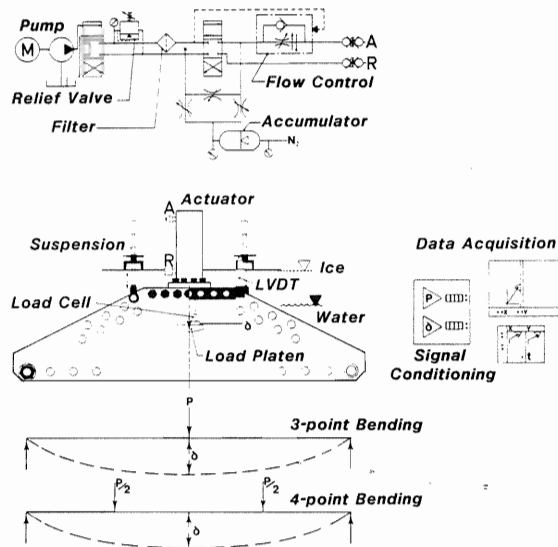
Fig. 2 Test frame schematic illustrating the hydraulic system and the loading geometry imposed on the beam specimen.
