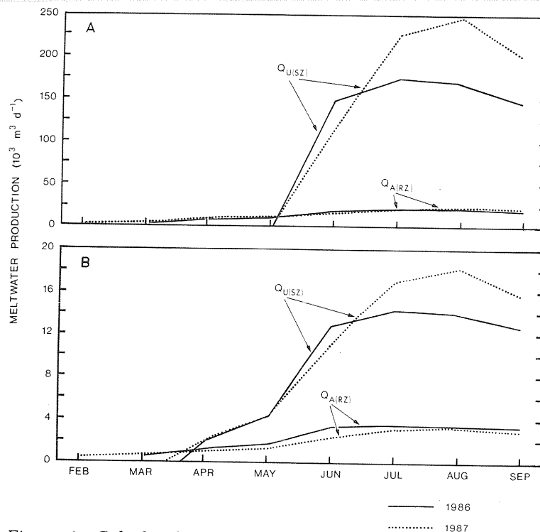
Figure 4: Calculated mean monthly rates of meltwater production from avalanche snow in the runout zone ( Q_{A(RZ)} ) and undisturbed snow in the starting zone ( Q_{U(SZ)} ) for two representative paths. Q_{A(RZ)} is based on the surveyed surface area of the avalanche deposits. A: 'Gorian' path; B: 'Saiful Maluk' path.
