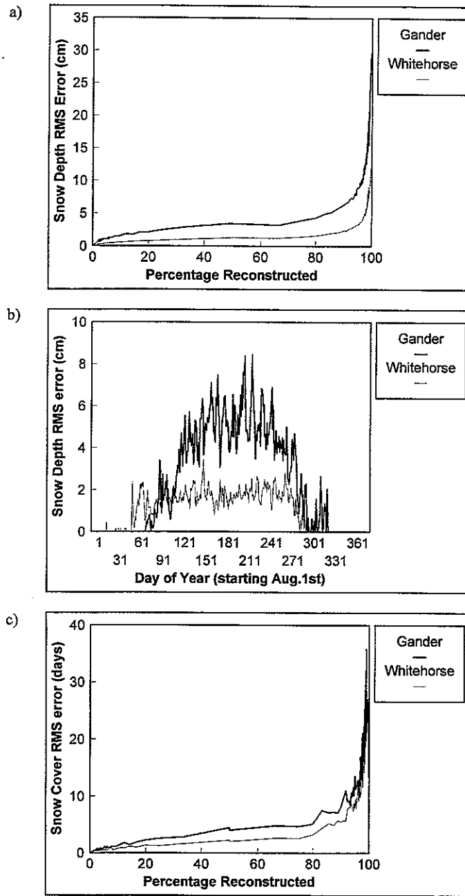
Figure 1: Snow depth reconstruction statistics for Gander and Whitehorse: a) total annual RMS error in snow depth reconstructions by proportion of data that is reconstructed; b) daily RMS error at the 86% reconstruction level (weekly observations); c) RMS error in snow cover duration reconstruction by proportion reconstructed.
