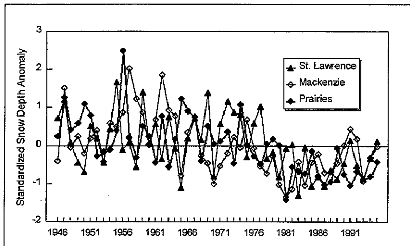
Figure 7: Temporal variation in mean winter (JFM) snow depth over three important snow depth response regions identified in the PC analysis. Snow depths are expressed as standardized anomalies.
