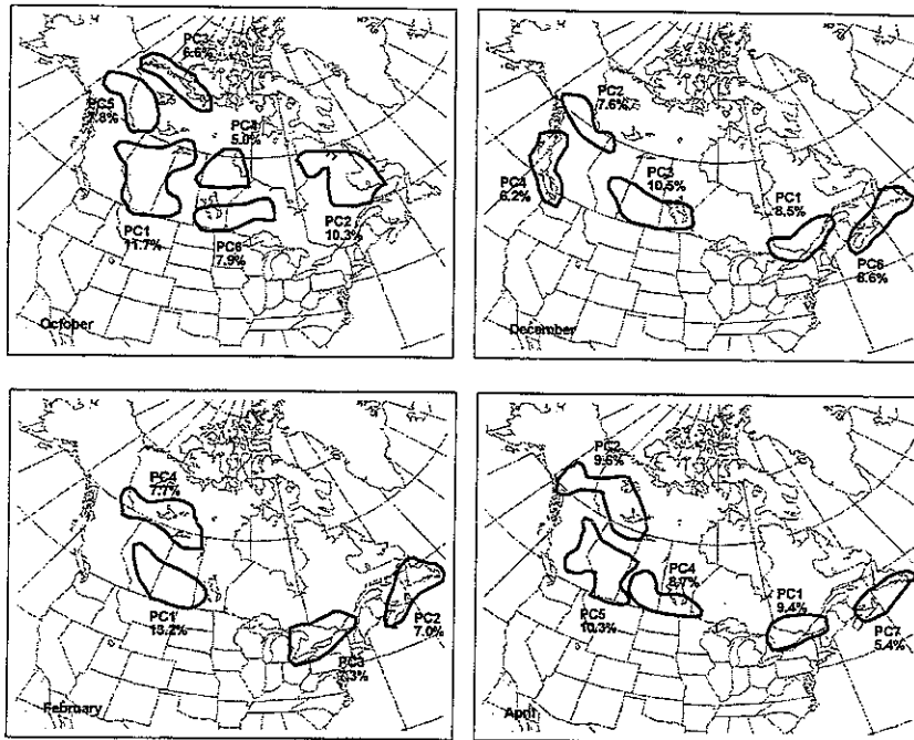
Figure 4: Location of PCs explaining more than 5% of the variance in monthly mean snow depth over the 1955-1995 period. Lines approximate the 0.7 contour of rotated PC loadings.
