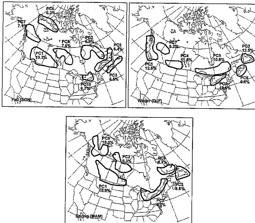
Figure 5: Location of PCs explaining more than 5% of the variance in seasonal snow cover duration over the 1955-1995 period. Lines approximate the 0.7 contour of rotated PC loadings. Results for the Summer (JJA) period are not shown as there were insufficient gridpoints to generate spatially consistent response regions.
