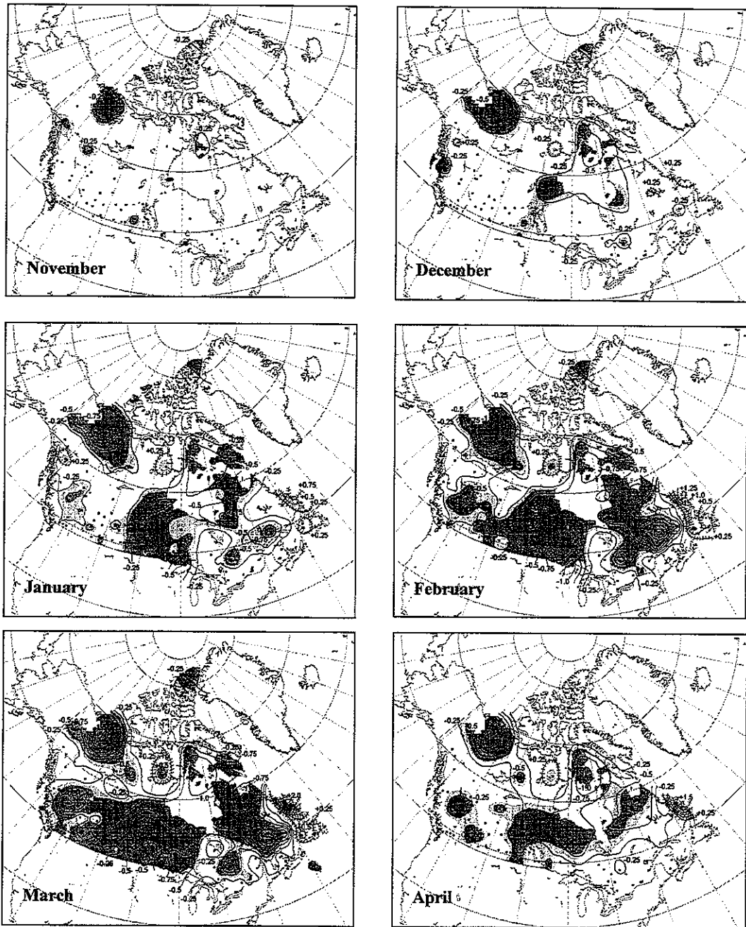
Figure 2: Average change in mean monthly snow depth over the 1946-95 period ( \text{cm.yr}^{-1} ). Increases are shown as cross-hatched contour lines and decreases as regular lines. The filled squares show the locations of the stations included in the analysis (were required to have at least 40 years of data in the period). Dark shading is used to highlight areas where changes in snow depth were locally significant ( p < 0.05 ). Light shading is used to highlight areas where station exhibited marginally significant ( 0.05 < p < 0.10 ) snow depth changes.
