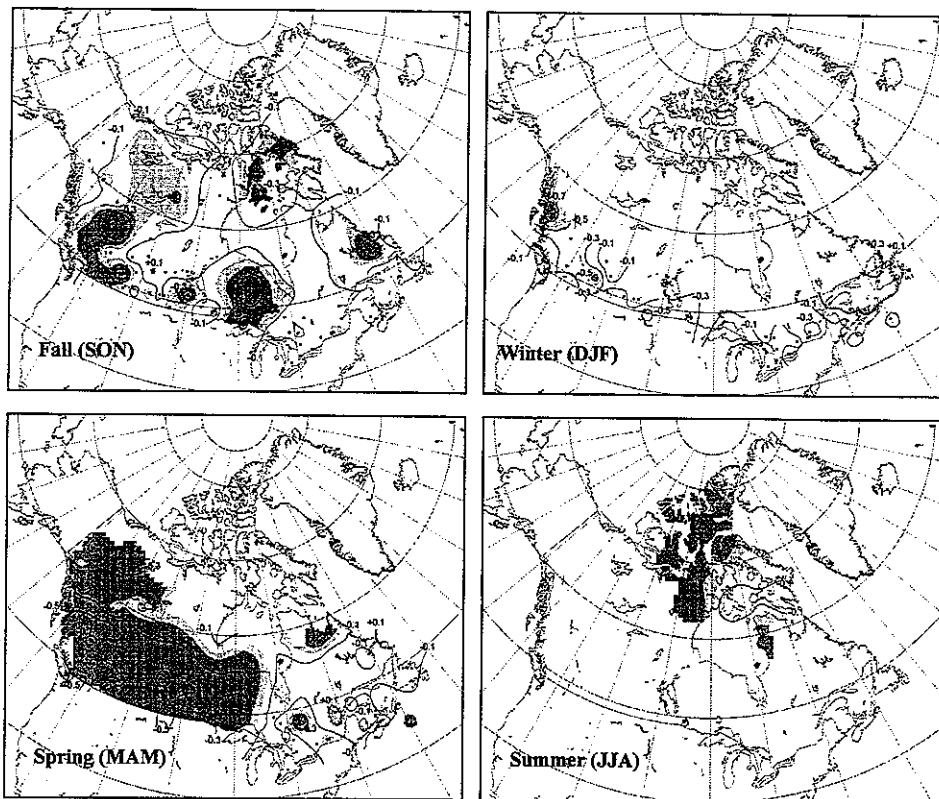
Figure 3: Average change in seasonal snow cover duration over the 1946-95 period (days.yr -1 ). See Figure 2 for explanation of shading.
