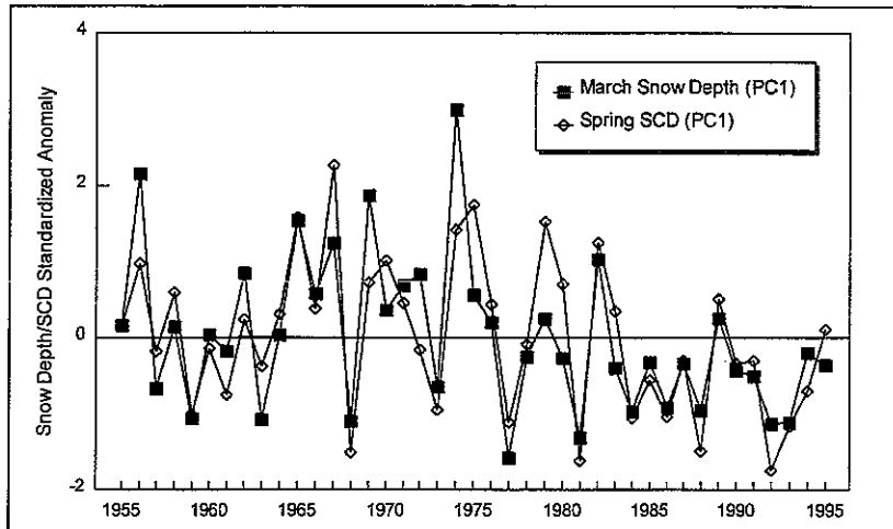
Figure 6: Comparison of March snow depth and spring snow cover fluctuations over the Prairie region. The correlation coefficient for both series is 0.8.
