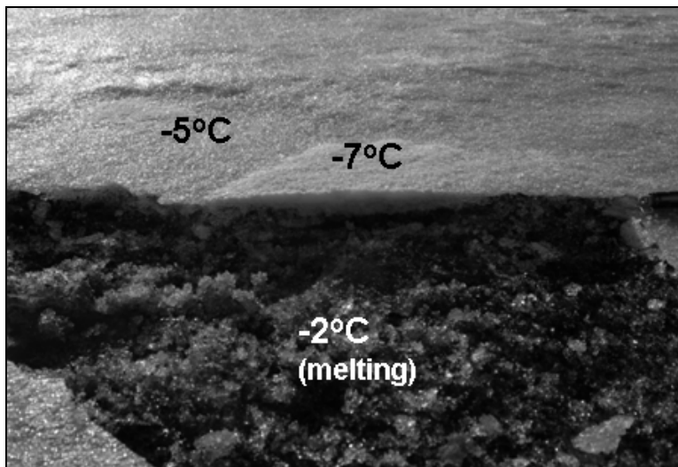
Figure 5. Observations of melting at negative air temperature conditions. Temperature were measured using an infrared temperature sensor, where the -7^{\circ}\text{C} area is snow, the -5^{\circ}\text{C} area is transparent ice and -2^{\circ}\text{C} is the BC-snow mixture below the surface. The air filled void between ice and BC-snow is approximately 3 cm thick.
