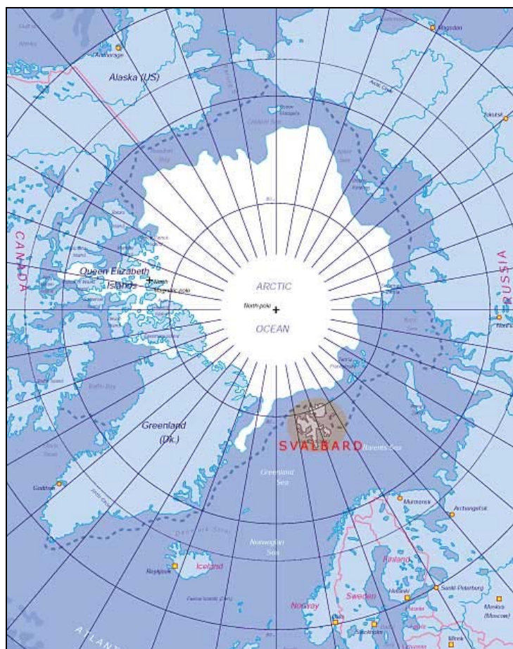
Figure 1. Geographical map of the north Atlantic including Svalbard, northern Europe and the Arctic Ocean.
