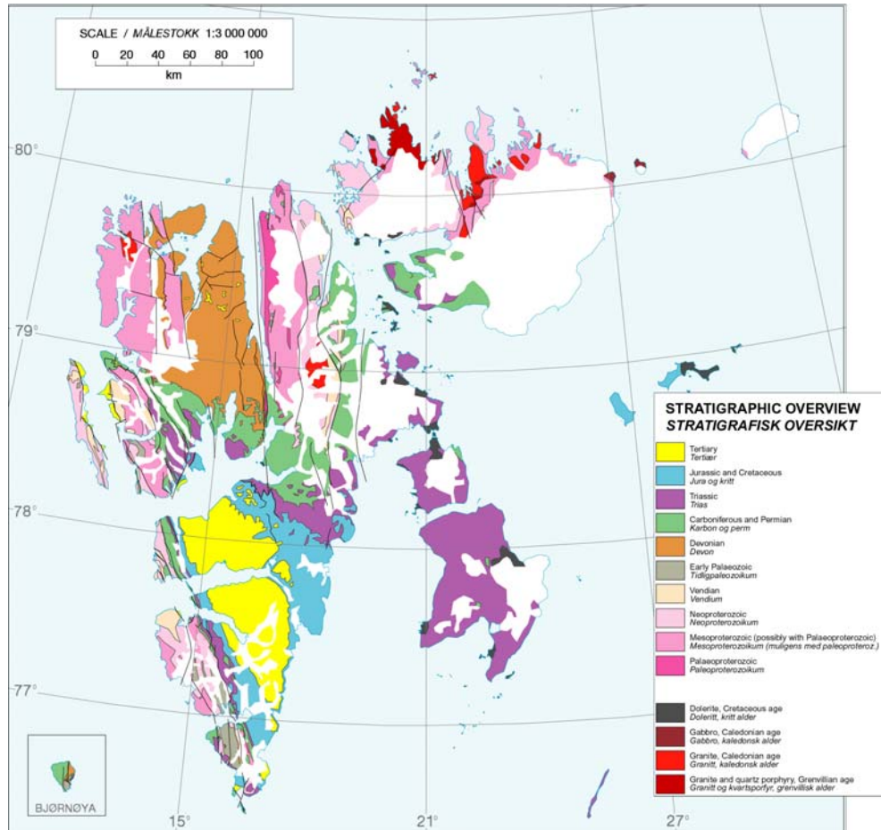
Figure 2. Geological map of Svalbard. Most coal deposits are found in the tertiary rock formations in the south-western Svalbard.
