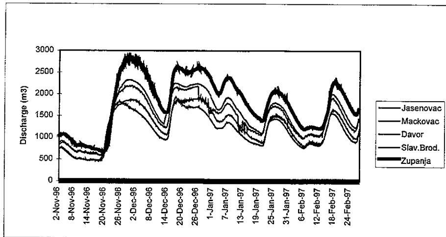
Fig. 3 - Dynamic stage rises along the mainstream of the Sava River during the winter of 1996-1997.
