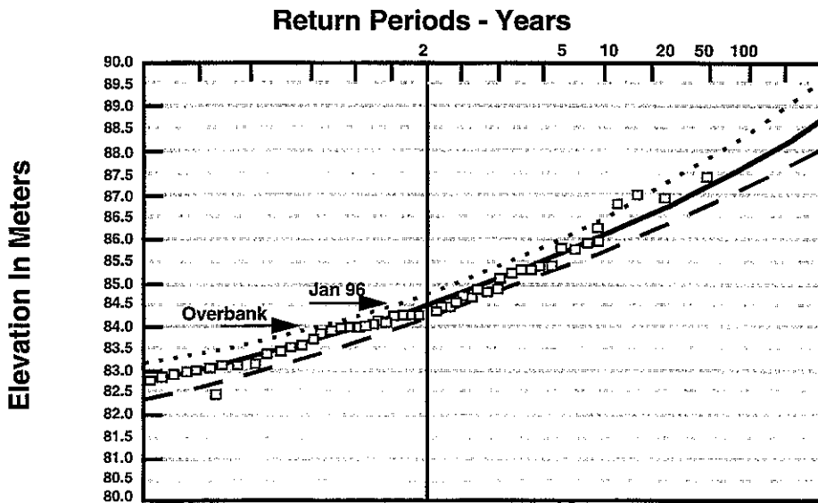
Fig. 2 - A frequency curve of peak events on the Sava River at Zupanja showing overbank floods occur in most winters.
