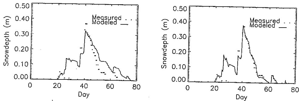
Fig. 4 - Losnica, Bosnia 1-D SNTHERM model runs with standard code (left) and with Bosnia version modifications (right).
