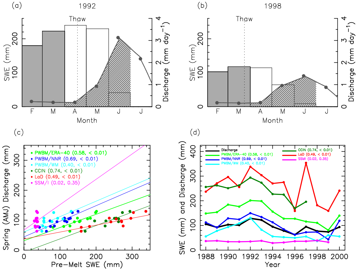
Figure 2: Monthly total SWE (mm) and mean discharge ( Q , \text{mm day}^{-1} ) across the Yukon basin for (a) 1992, a year with relatively high SWE and Q , and (b) 1998, a year with low SWE and Q totals. Vertical bars show SWE— in this case from PWBM driven with ERA-40 data (PWBM/ERA-40). February and March SWE values (gray bars here) are averaged to give “pre-melt” SWE in this study. April–June SWE are depicted by white bars. Spring Q (monthly values indicated by dots at middle of month) is the integration of the monthly Q for April through June (hatched area), and is used for comparisons with the pre-melt SWE. A “thaw date” (marked Thaw) estimated from SSM/I data are used in alternate Q integrations. (c) Scatterplot of pre-melt SWE from each data set, for years 1988–2000. The best fit line based on linear least squares regression is shown. (d) Time series of SWE and Q . Statistics ( R^2 and associated p -value) for each covariance comparison are shown in parenthesis.
