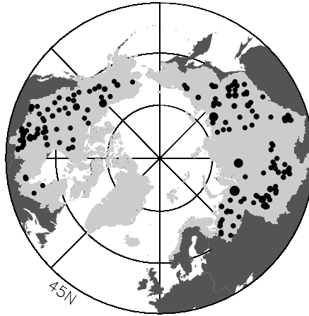
Figure 1: Pan-Arctic land mass (north of 45°N, dark gray), the arctic drainage basin (light gray), and locations of 179 river basins used in the study. Dot sizes are scaled by basin area. A total of 39,926 EASE-Grid cells comprise the approximately 25 million km 2 drainage basin. Areas for the 179 river basins range from 20,000 km 2 to 486,000 km 2 .
