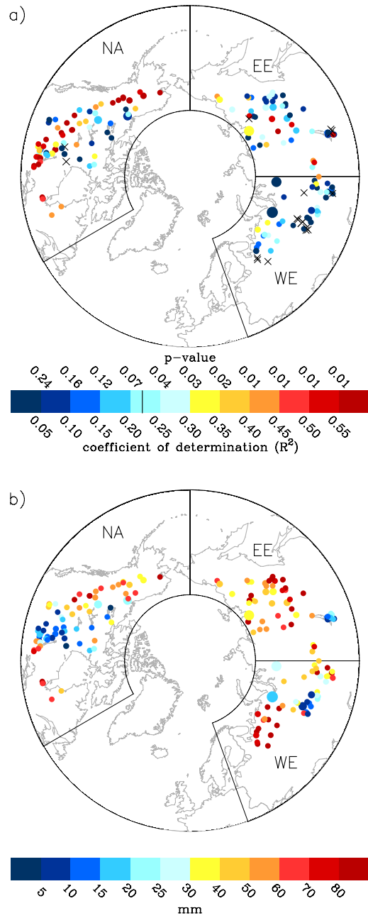
Figure 4: (a) R^2 for PWBM simulated spring total Q vs. observed spring total Q . The vertical line in colorbar is level at which R^2 is significant. Minimum, maximum, and mean R^2 s across all basins, North America (NA), western Eurasia (WE), and eastern Eurasia (EE) are shown in Table 1. The 'X's mark basins with a negative correlation. (b) Standard deviation of spring (April–June) discharge for the period 1988–2000.
