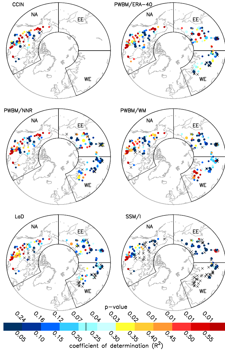
Figure 3: Explained variance ( R^2 ) for pre-melt SWE and spring Q comparisons (1988–2000) at the 179 river basins and for the 6 SWE products. SWE is taken from the CCIN SWE analysis; PWBM simulations driven by ERA-40, NNR and WM; LaD model; and SSM/I data. The 'X's mark basins with a negative correlation. Average R^2 values across all basins, North America (NA), western Eurasia (WE), and eastern Eurasia (EE) are shown in Table 1. The vertical line in colorbar is level ( R^2 = 0.22 ) at which R^2 is significant at 5% level. P-values associated with each R^2 interval are shown above the colorbar. Note that p < 0.01 for all R^2 \geq 0.40 .
