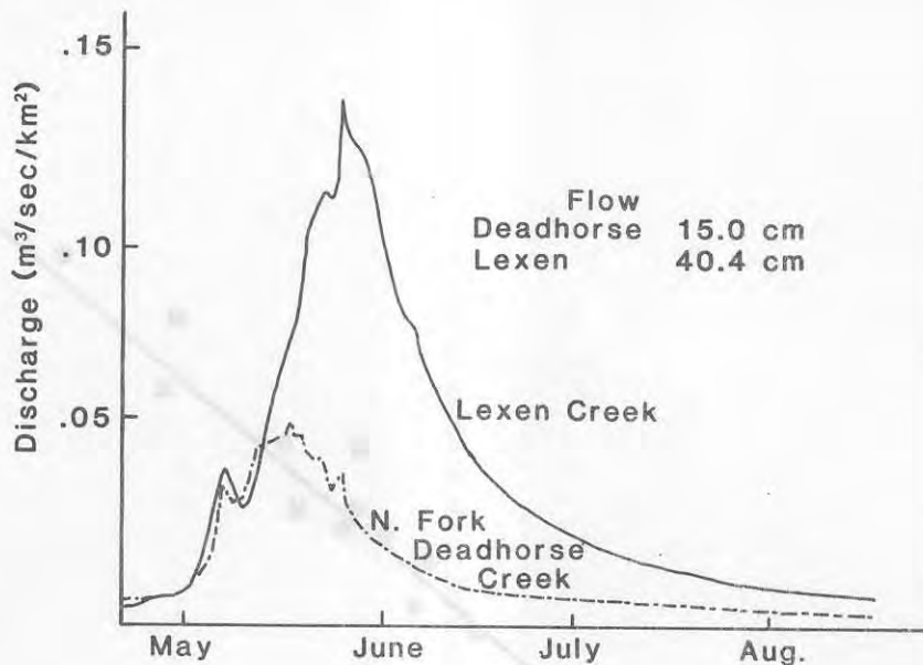
Figure 2.--Comparative hydrographs from North Fork and Lexen Creeks for an average year prior to harvest on the North Fork.
