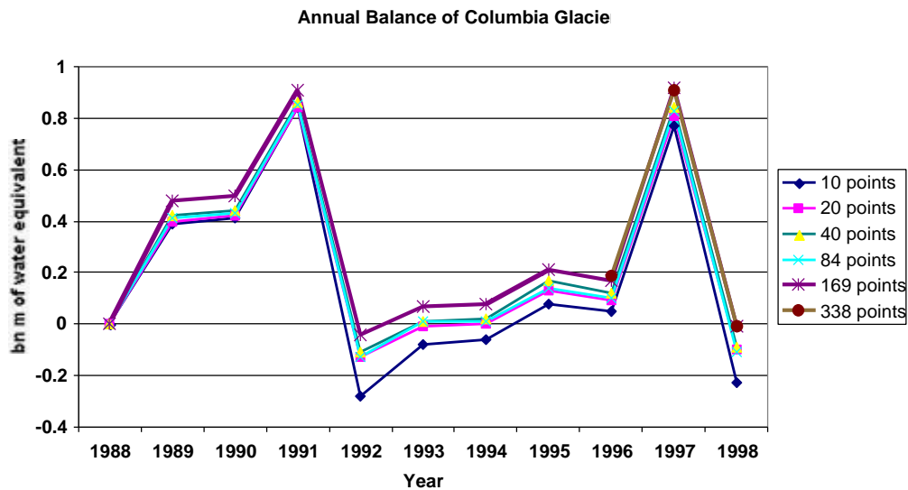
Figure 4. Annual balance of Columbia Glacier.
