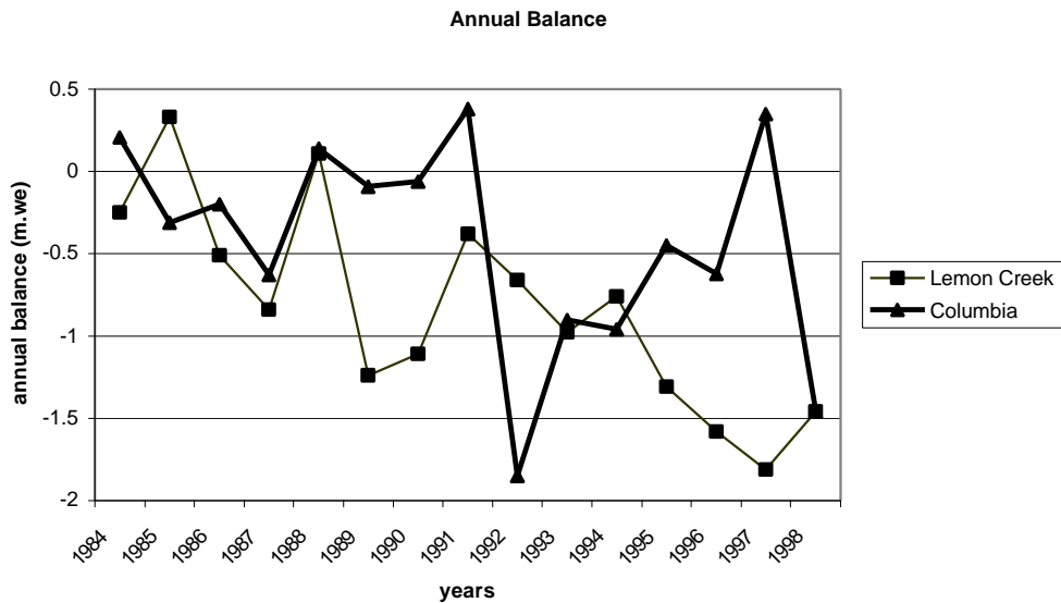
Figure 3. The annual balance of Columbia and Lemon Creek Glacier Alaska in meters of water equivalent.
