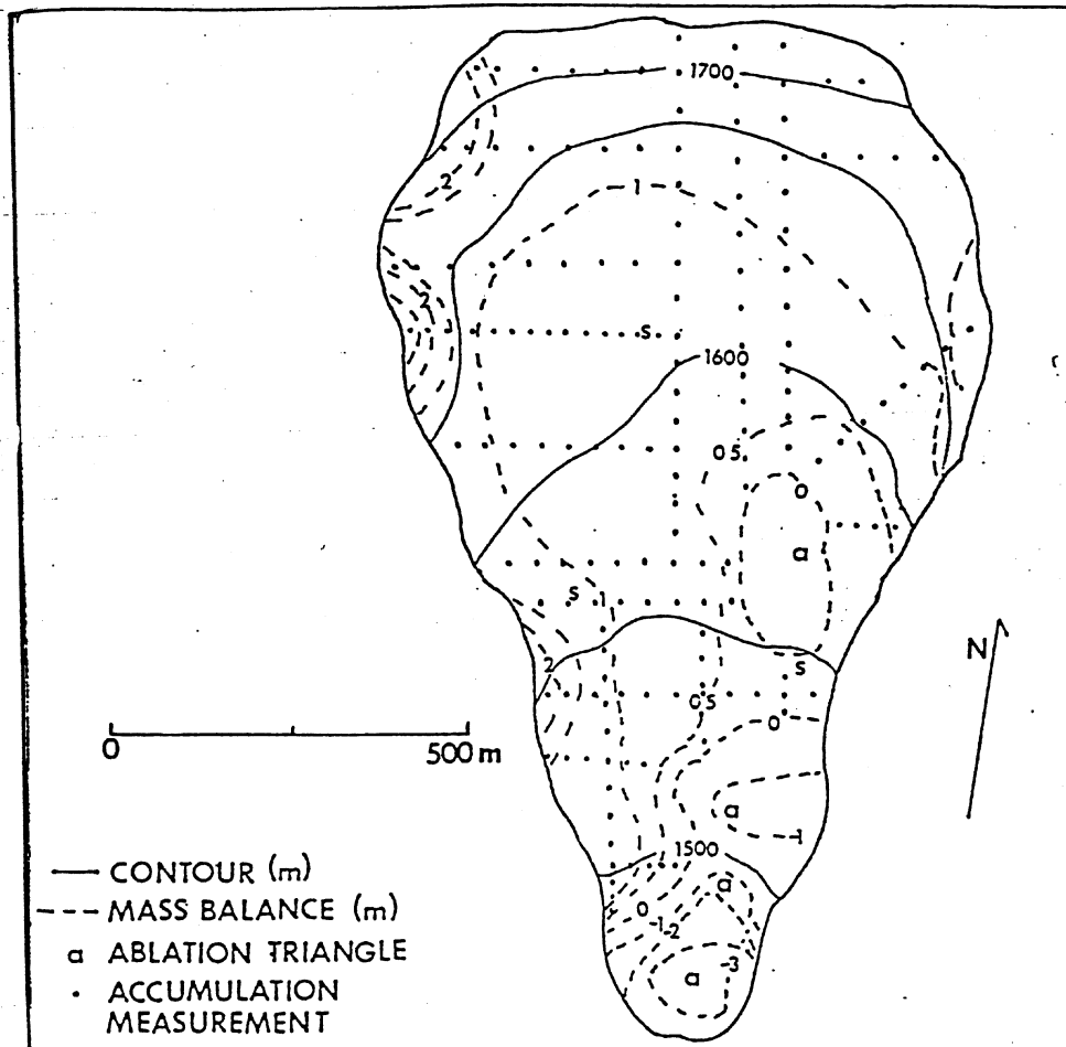
Figure 1. Mass balance map of Columbia Glacier.
