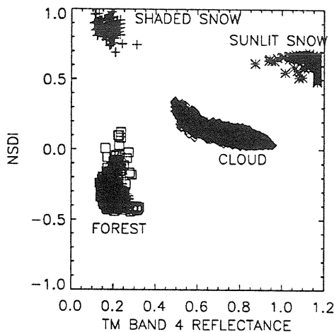
Figure 1. Relationship of NSDI to TM band 4 reflectances for four features sampled from a Landsat TM image of the Brooks Range, Alaska.
