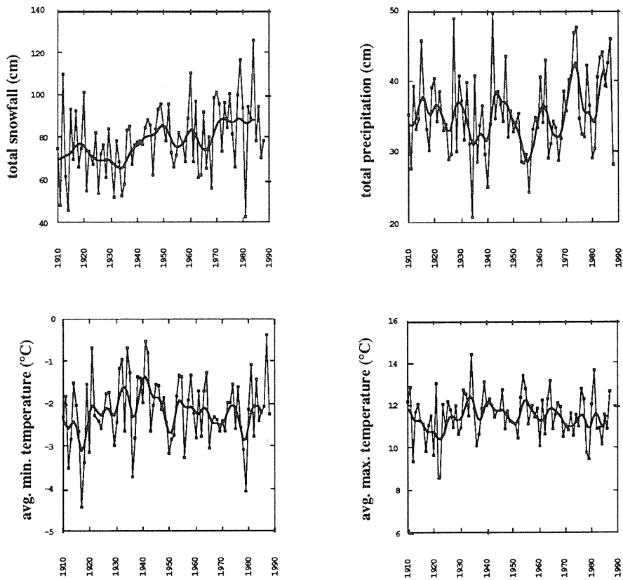
Figure 5. Total snowfall (cm), total precipitation (cm), average minimum temperature ( ^{\circ}\text{C} ), and average maximum temperature ( ^{\circ}\text{C} ) for the Great Plains region for September-May 1909/10 through 1987/88. The data were smoothed using a 9-point binomial filter.
