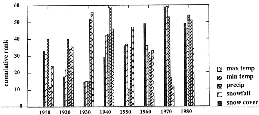
Figure 6. Cumulative rank among snow cover, snowfall, precipitation, and maximum and minimum temperature for the Great Plains region. Data were averaged by decades for each sub-region and ranked from 1 (lowest) to 8 (highest). The ranks were summed to get a region-wide decadal rank.
