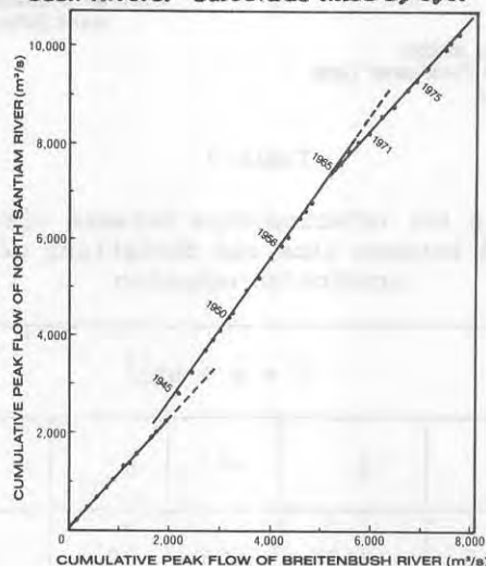
Double-mass plot of cumulative peak flows of the North Santiam and Breitenbush Rivers. Curve was fitted by eye.
