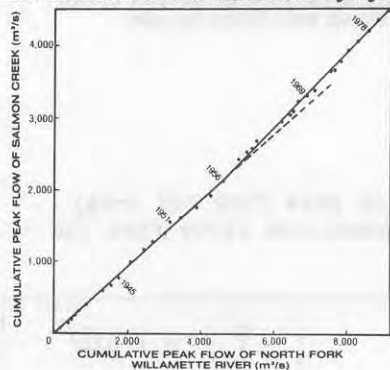
Double-mass plot of cumulative peak flows of Salmon Creek and the North Fork of the Willamette Middle Fork. Curve was fitted by eye.
