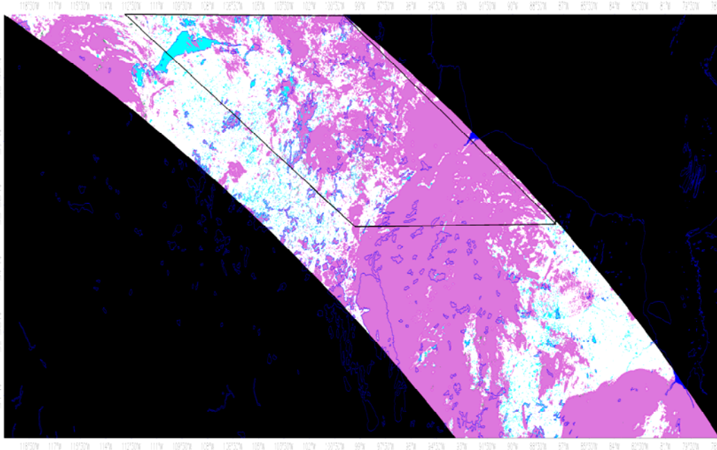
Figure 2. MODIS snow map, 500 m resolution, of the boreal study area on 10 April 2008, tile h12v03 with the study area outlined (black polygon). Snow is white, snow and ice covered lakes are blue-green, clouds are pink. The image shown is mapped in geographic projection. The star shows the approximate location of Thompson Zoo, Manitoba weather station.
