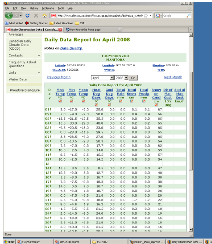
Figure 5. Daily data report April 2008, Thompson Zoo, Manitoba.
