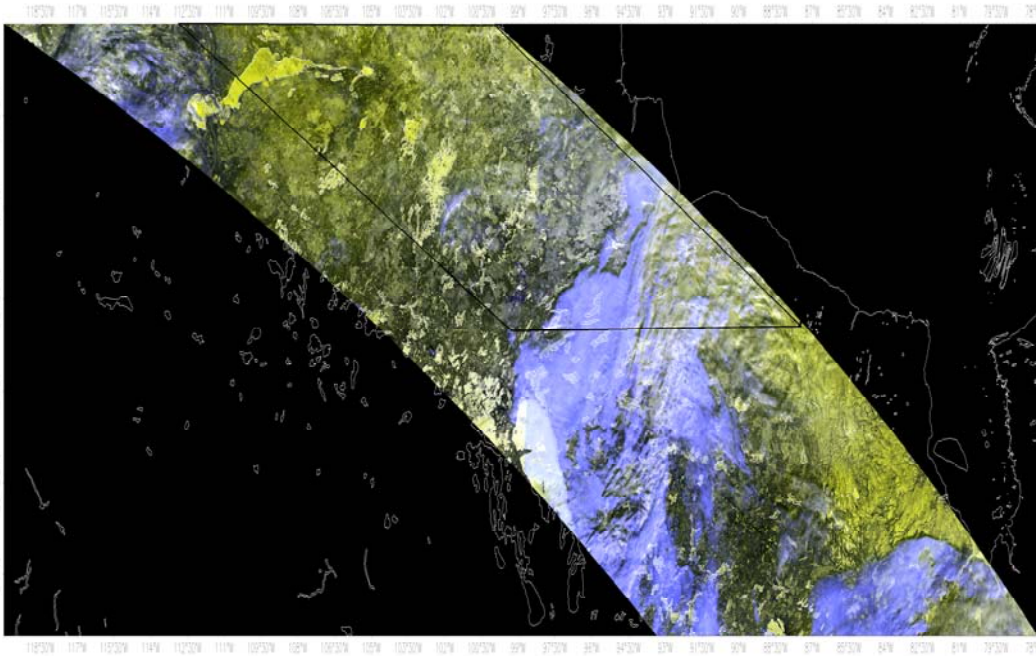
Figure 1. View of the boreal study area shown as MODIS bands 1, 4, 6 RGB image to highlight the presence of snow. Snow appears yellow in this band combination, pixels dominated by snow are brightest yellow; snow mixed with other surface features appears in decreasing shades of yellow. Clouds appear in white and light gray over some surface features. The study area is outlined (black polygon). Date of image is 10 April 2008; the daily surface reflectance product MOD09GA, tile h12v03, 500 m resolution, mapped in geographic projection. The star shows the approximate location of Thompson Zoo, Manitoba weather station.
