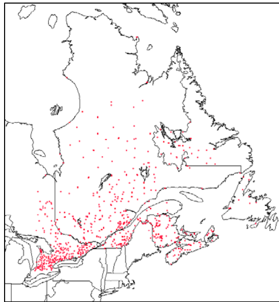
Figure 1. Location of snow course observations with complete observations of March 01 SWE during the decade of the 1970s.
