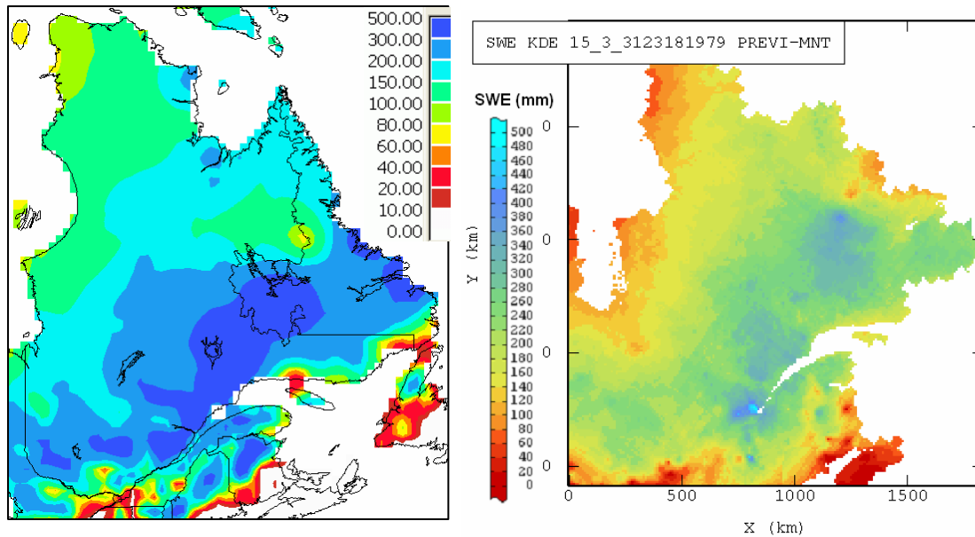
Figure 4. Comparison of SWE maps for March 15, 1979 from Brown et al. (2003) (left) and the KED method (right).
