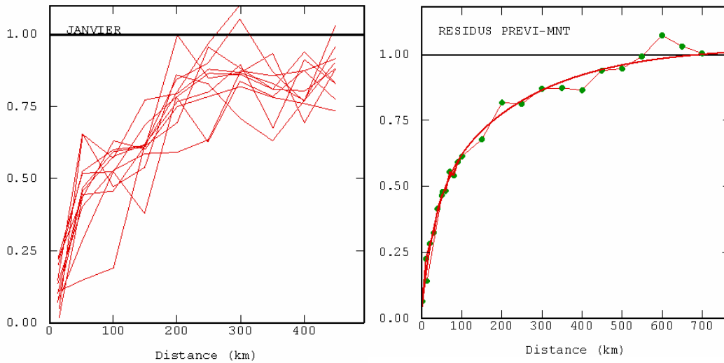
Figure 3. Construction of the mean normalized variogram (right) from annual variograms for January 01 SWE from 1970 to 2005 (left).
