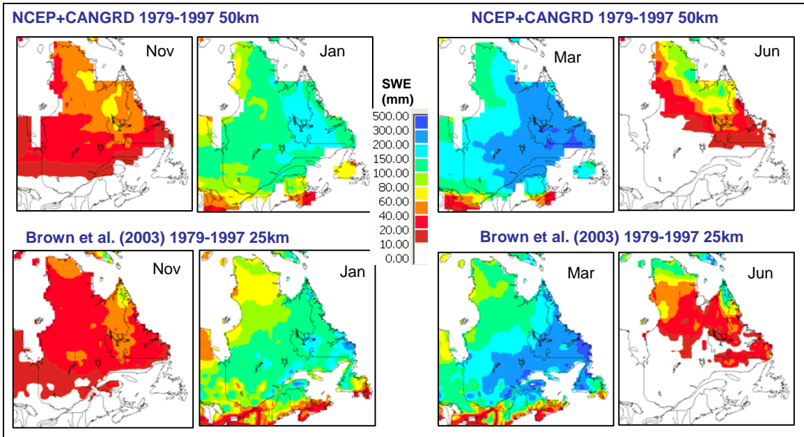
Figure 2. Comparison of the reconstructed SWE monthly climatologies (NCEP+CANGRD) with the Brown et al. (2003) dataset for the 1979-1997 period.
