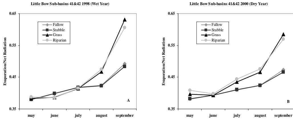
Figure 2. Evapotranspiration Efficiency (E-Ratio) determined for wet (A) and dry years (B) for the Little Bow watershed sub-basins 41 and 42. The larger the LE/R_n the more 'productive' the vegetative cover. LE/R_n is lowest in May and greatest in September as the ground warms. LE/R_n is similar in Spring for both years but is higher in the wet year by the end of Summer.
