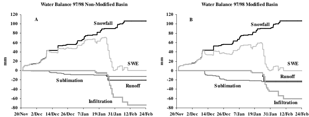
Figure 1. Modelled water balance results for the Little Bow watershed, sub-basins 41 and 42 for original (A) and modified (B) HRU scenarios.
