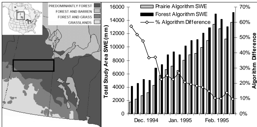
Figure 2. Comparison of current MSC land-cover sensitive algorithm and previous MSC algorithm that does not consider land cover. Graphic on left illustrates the study area for which total SWE was calculated.
