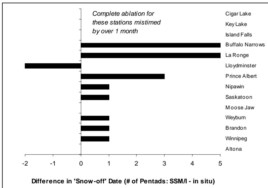
Figure 3. Comparison of snow-off timing between the passive microwave and in situ SWE datasets.
